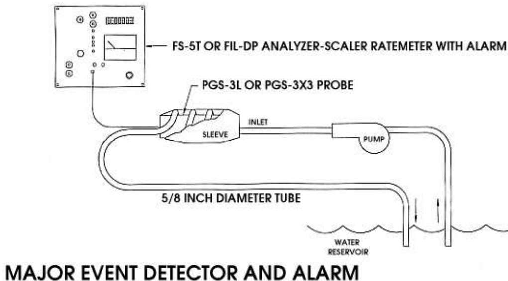
Figure 1: FS-5T(Top); PGS-3L(Bottom)
